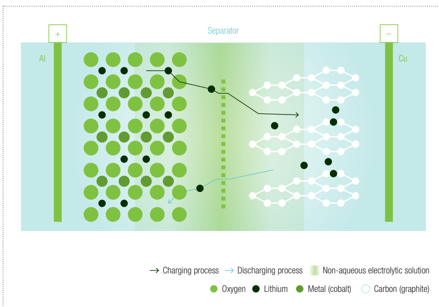
Schematic structure of a lithium-ion cell (positive electrode: \text{LiCoO}_2 ; negative electrode: Li graphite)
