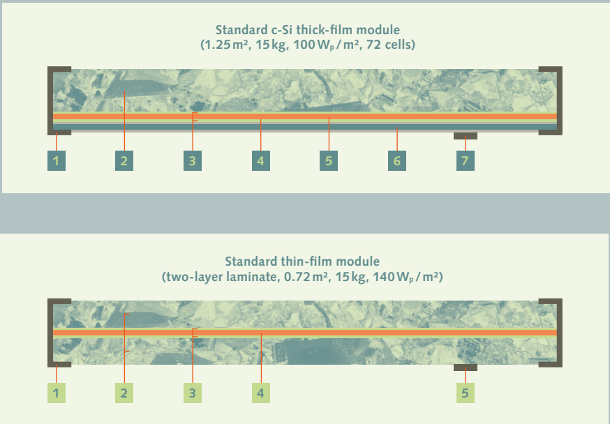
Figure 1: Standard designs of thick- and thin-film PV modules
