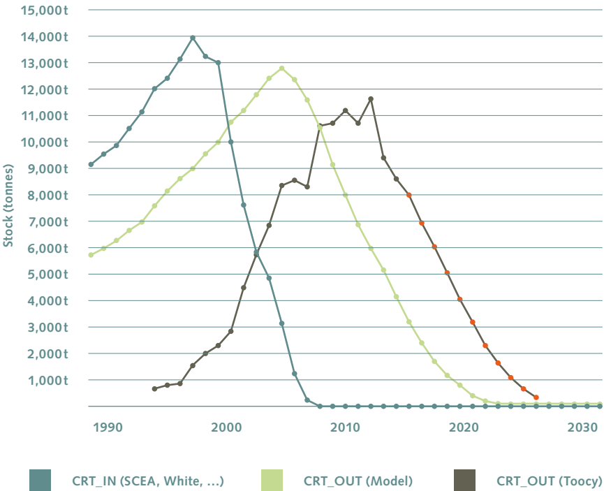
Model and measurement data of Swiss CRT glass flows in tonnes per year. Data for the return "CRT_OUT (Toocy)" was collected up to 2014, from 2015 (●) onwards it was estimated. Data for "CRT_IN (SCEA, White, ...)" concerns sales figures from 1995 (TVs) and from 1985 (PCs). "CRT_OUT (Model)" shows the return already simulated in 2006. The simulation used a Gaussian distributed market retention of CRTs to their final disposal ( \mu = 10 ; \sigma = 3 for TVs, and \mu = 7 ; \sigma = 1.5 for PCs). The real return is delayed by around five years, and the mean retention time for TVs has been calibrated to 15 years ( \mu = 15 ).
