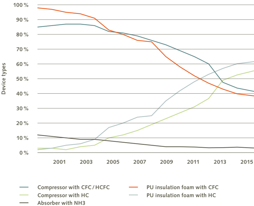
Figure 1: Development of the device types processed at stage 1 (CFC- / HCFC- and HC-containing compressors, ammonia-containing absorption systems) and stage 2 (CFC- and HC-containing PU insulation foam).
